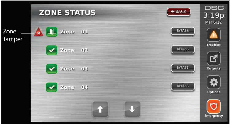
Figure 8 - Zone Tamper
