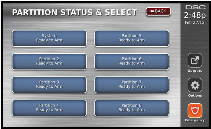
Figure 15 - Partition Status
